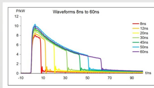
150W/200W M7波形图 150W/200W M7 Waveform Graph
