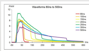
150W/200W M7波形图 150W/200W M7 Waveform Graph
